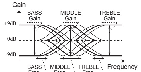
Diagram of 3-bands Equalizer
